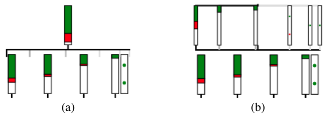
Fig. 8. Detail view of the third claim and its children in Fig. 7 (top) (a) showing the normal node and (b) analyzing the probabilities of its positions by replacing it with multiple, slimmer subnodes for each position: the claim occurs most often before all its children but may occur at any other position as well (with far smaller probability).
