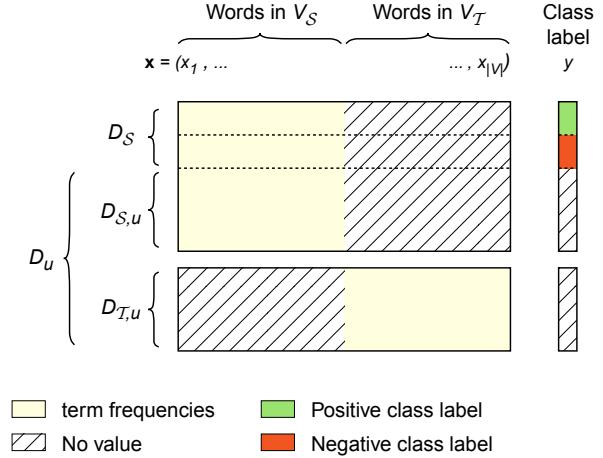
Figure 1: The document sets underlying CL-SCL. The subscripts \mathcal{S} , \mathcal{T} , and u designate “source language”, “target language”, and “unlabeled”.
