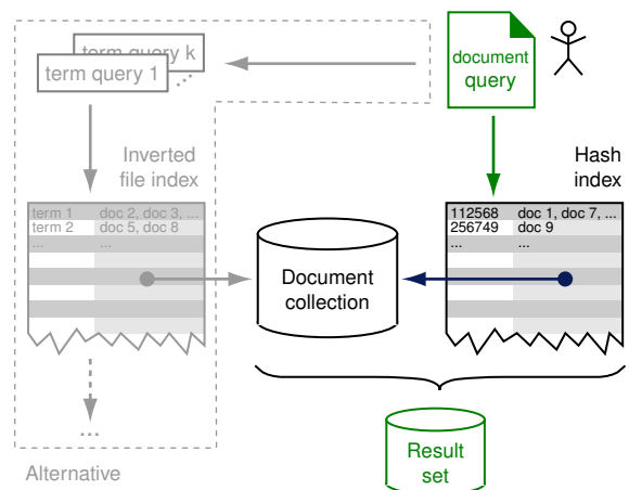
Figure 3: Illustration of a similarity search retrieval task. Starting point is an information need formulated as document query, which is satisfied with a hash index in constant time of the document collection size. Alternatively, keywords may be extracted from the document query to formulate several term queries.
