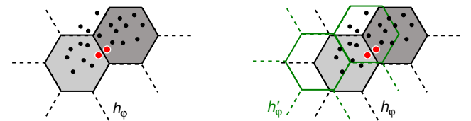
Figure 6: A set of documents projected in the two-dimensional space. A hash function h_\varphi partitions the space into regions that are characterized by different hash keys. Even if two documents (colored red) are very similar to each other they may be mapped onto different hash keys (left). This threshold-behavior can be alleviated by employing several functions h_\varphi and h'_\varphi (right).
