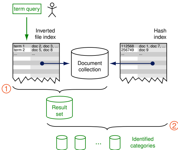
Figure 2: Illustration of a grouping retrieval task. Starting point is an information need formulated as term query, which is satisfied with an inverted file index, yielding a result set (Step ①). The subsequent categorization is realized with a hash index in linear time of the result set size (Step ②).
