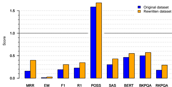
Figure 2: Highest scores reached per dataset variant for each metric. For all metrics except POSS a score of 1 corresponds to optimal performance.
