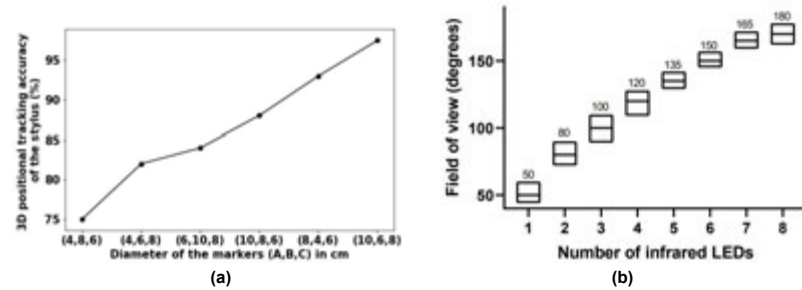
Fig. 5. (a) Diameters of markers A,B,C vs. 3D tracking accuracy and (b) Number of infrared LEDs vs. field-of-view.
