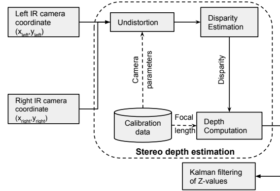
Fig. 8. Overview of RetroSphere's Stereo depth estimation pipeline.
