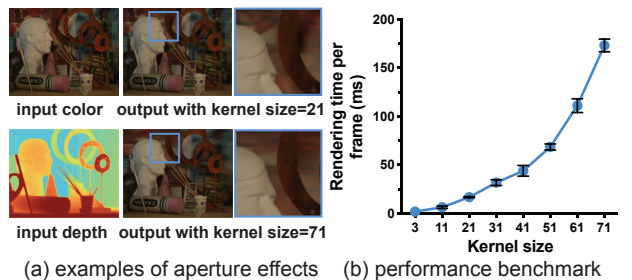
Figure 16. Examples and performance evaluation of real-time aperture effects. (a) shows a pair of input color and depth images and the corresponding results with Gaussian kernel sizes of 21 and 71 in Algorithm 3. (b) shows a performance evaluation with real-time camera images on a Pixel 3. According to the results, we recommend a kernel size of 11-21 to deploy our real-time wide-aperture effect on Pixel 3 or comparable mobile devices.
