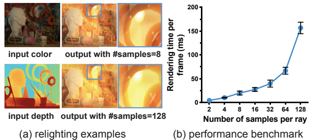
Figure 15. Examples and performance evaluation of real-time relighting. (a) shows a pair of input color and depth images and the corresponding results with 8 and 128 samples per ray in Algorithm 3. (b) shows a performance evaluation with real-time camera images on a Pixel 3. According to the results, we recommend 4-8 samples per ray to deploy our relighting module on Pixel 3 or comparable mobile devices.
