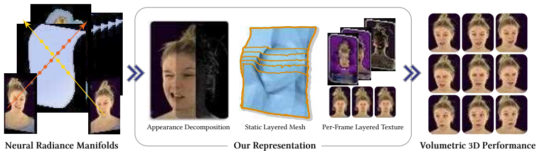
Fig. 1. We model a dynamic face sequence as a set of radiance manifolds, which are exported as a static layered mesh and an animated texture. This allows for smoothly controlling the quality vs. memory and compute footprints, while achieving efficient and photorealistic rendering of volumetric scenes using established graphics pipelines without any neural network integration.
