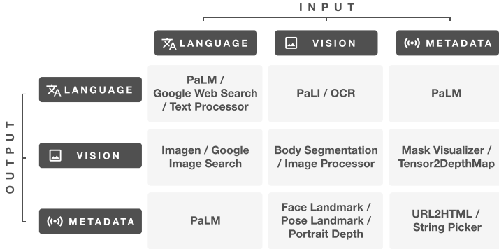
Fig. 3. An overview of major primitive processor nodes supported by InstructPipe. 17 of the 20 processor nodes are categorized by the type of accepted I/O into a 3 × 3 matrix. Note that “PaLM” represents two nodes in InstructPipe, i.e. , a text generation model and a chat model of PaLM [3].
