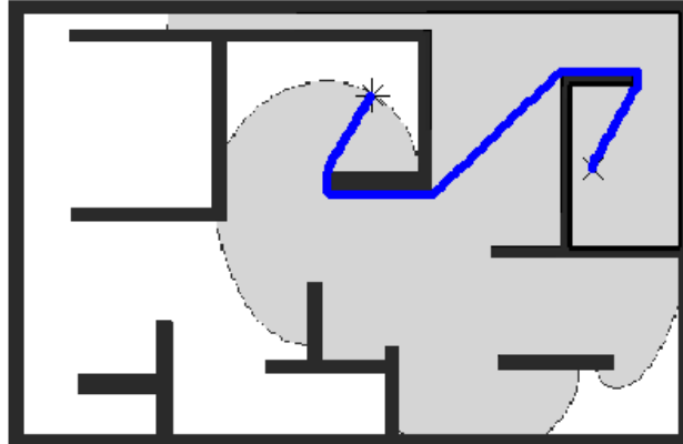
Figure 1: Trajectory calculated by the Fast Marching method directly.
