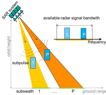
Fig. 1. Transmitted subpulses.
