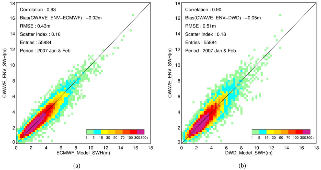
Fig. 7. Scatter plots of SWH derived by CWAVE_ENV compared to (a) the ECMWF reanalysis model and (b) the DWD forecast model for data acquired in January and February 2007.
