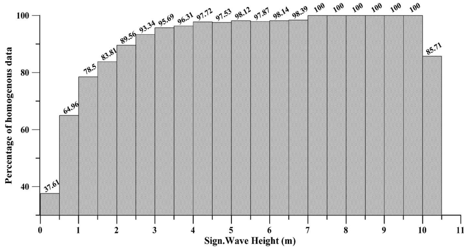
Fig. 6. Percentages of the ASAR wave mode data that pass the homogenous test in different sea states acquired during January–February 2007.
