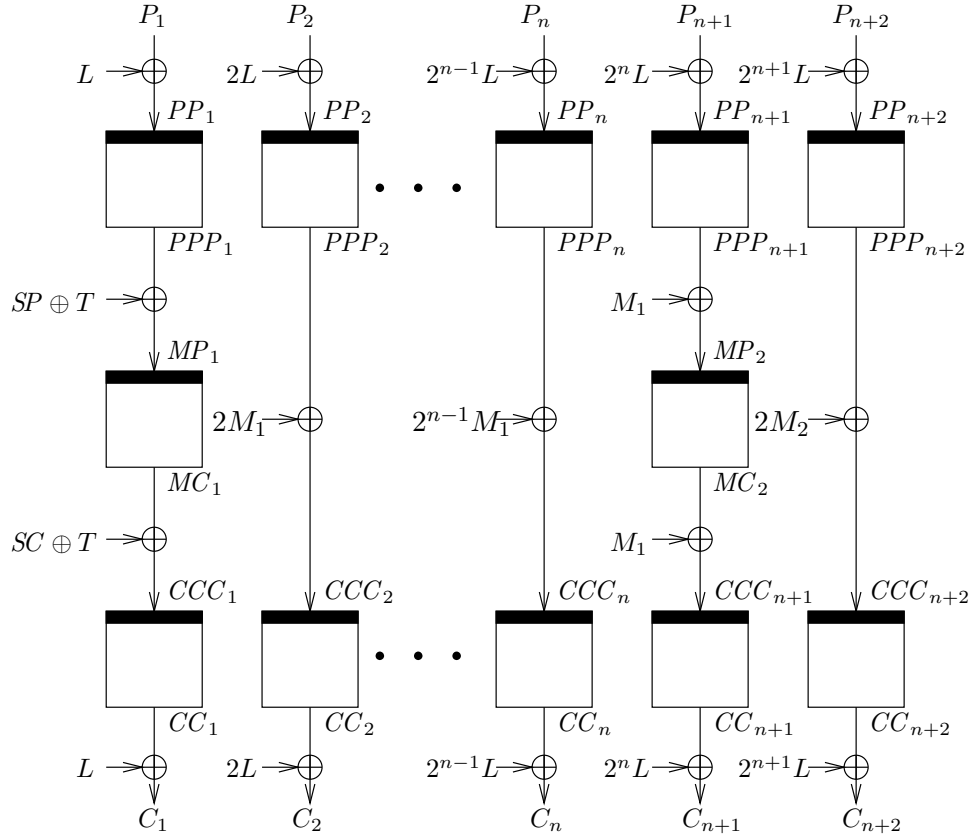
Figure 4: Enciphering an (n+2) -block message under \text{EME}^+ . The boxes represent E_K and L = 2E_K(0^n) . We set SP = PPP_2 \oplus \dots \oplus PPP_m , M_i = MP_i \oplus MC_i , and SC = CCC_2 \oplus \dots \oplus CCC_m .
