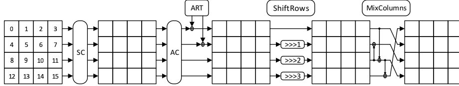
Fig. 1. The SKINNY round function
