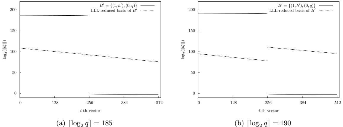
Fig. 1: Plots of \log_2(\|b_i^*\|) for the subfield lattice B' = \{(1, h'), (0, q)\} and \log_2(\|b_i^*\|) for the LLL-reduced basis of B' .
