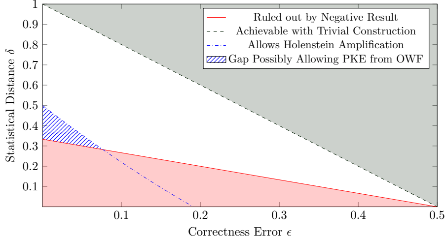
Figure 1: The graph gives an overview over the possible range of parameters for sacO. In the upper right are parameter regimes that can be achieved using the construction described in Appendix A. In the lower left are the strong parameter regimes ruled out by our negative result in Section 3. The graph shows nicely the gap between the parameters that can be ruled out and those that can be used to construct public key encryption using the construction of Sahai and Waters as well as the amplification technique of Holenstein.
