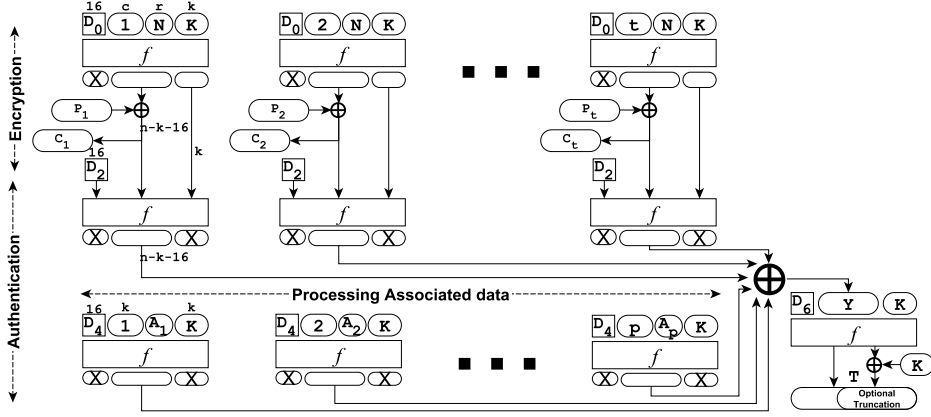
Fig. 1: Encryption and Authentication with PAEQ
