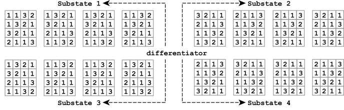
Fig. 6: Byte Inter-relations after \mathcal{R}_{19} \leftrightarrow Location of differentiator fault.
