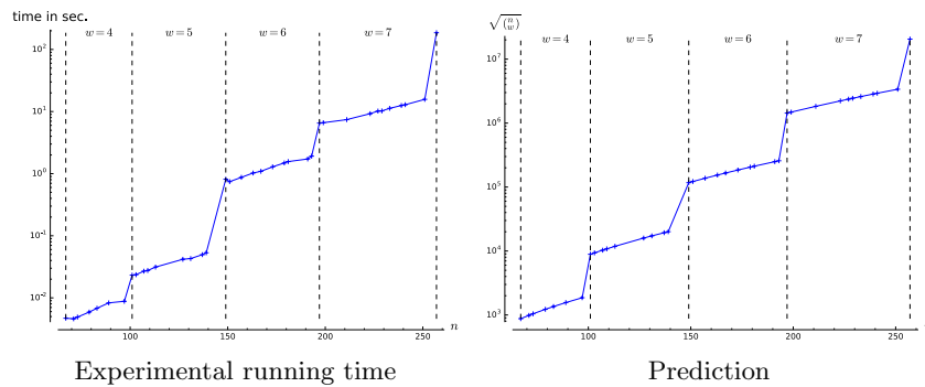
Fig. 3. Average running time of the classical attack over 100 trials in comparison with the function \sqrt{\binom{n}{w}} , which is the dominant factor in our asymptotic complexity.
