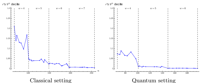
Fig. 1. 9 th decile of the ratio between the measured number of collisions c and expected number of collisions c' according to Heuristic 2, over 100 experiments per dimension.
