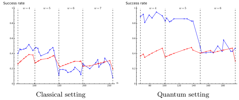
Fig. 2. Success rate of the attack over 100 trials (in blue), compared to the theoretical success rate (1 - 2w/(n - B))^B (in red). The rather discontinuous shape of the red curve is due to the rounding of w = \lfloor \sqrt{n}/2 \rfloor and B = \lfloor \log_2 \binom{n-1}{w-1} \rfloor .
