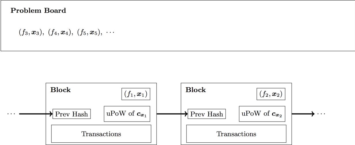
Figure 1: We present a framework for Blockchain to use uPoWs. Delegators post to a public Problem Board from which workers grab problems to mine a block with by producing a Proof of Useful Work that they attach to the block.
