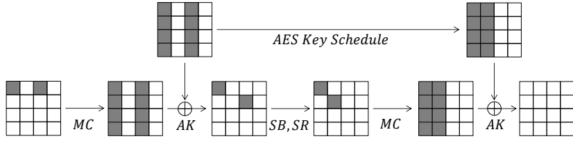
Figure 2: An example of linear incompatibility for 2-round AES in [FJP13, Figure 7].
