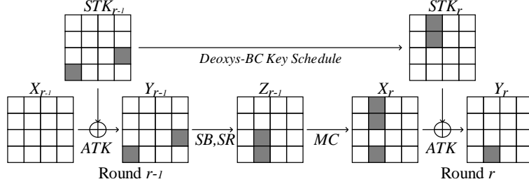
Figure 3: An example of consumption degrees Type 2.
