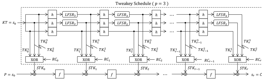
Figure 1: Instantiation of the TWEAKEY framework for Deoxys-BC-384.
