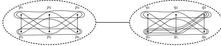
Fig. 1: The access structure \mathcal{F} \cdot \overline{\mathcal{F}} = \Gamma[a \rightarrow \mathcal{F}][b \rightarrow \overline{\mathcal{F}}] where \Gamma = ab (see Example 3). Also, it can be viewed as \mathcal{F} \cdot \overline{\mathcal{F}} = \Gamma[p_7 \rightarrow \mathcal{F}] where \Gamma = \mathcal{F} \cdot p_7 (see Remark 2). See Example 2 for descriptions of \mathcal{F}, \overline{\mathcal{F}} and \mathcal{F} \cdot \overline{\mathcal{F}} .
