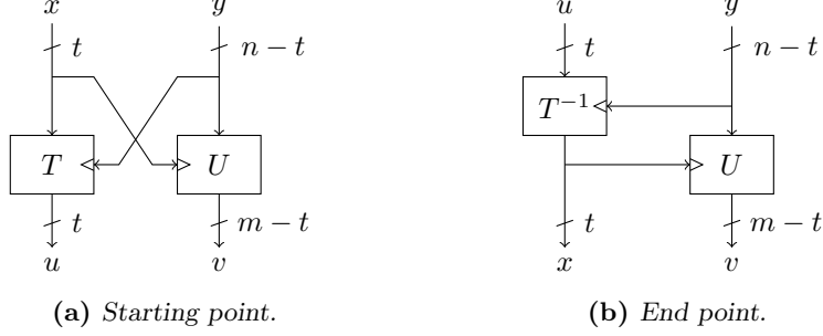
Figure 3: Function twisting.
