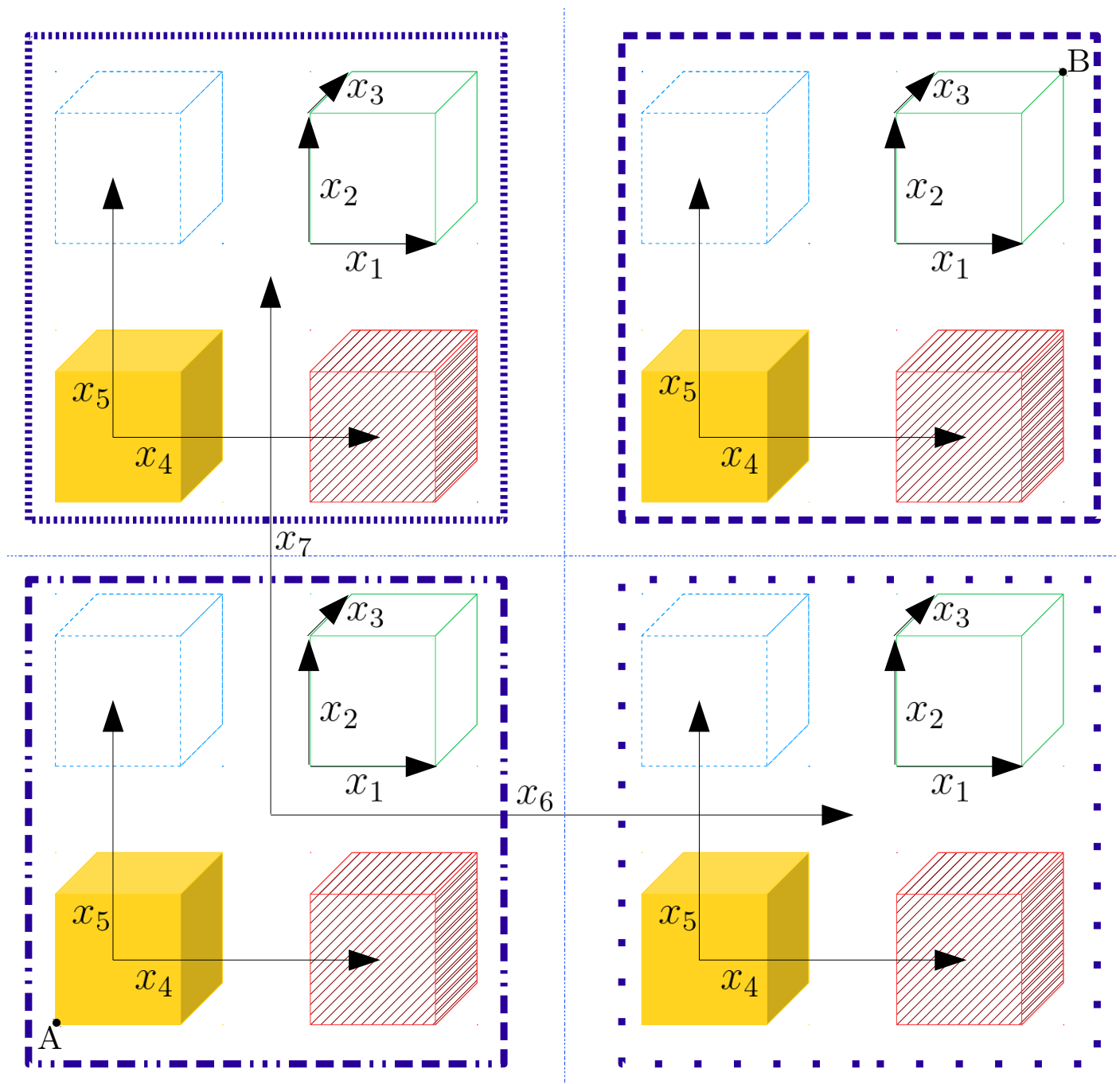
Figure 4. Representation of the hypercube structure of the group of automorphisms available in the multivariate polynomial RLWE with \Phi_4(\cdot) as polynomial functions and considering 7 independent variables \{x_1, \dots, x_7\} .
