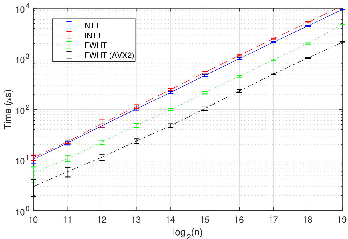
Figure 2. Runtimes of the proposed FWHT compared to the NTT/INTT from [6].
