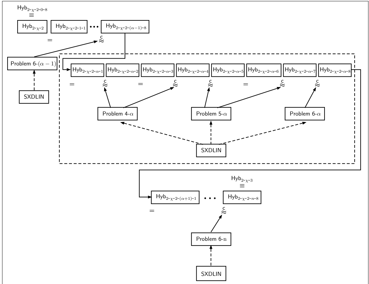
Fig. 4.2: Structure of the Hybrid Reduction for the Proof of Lemma 4.5
