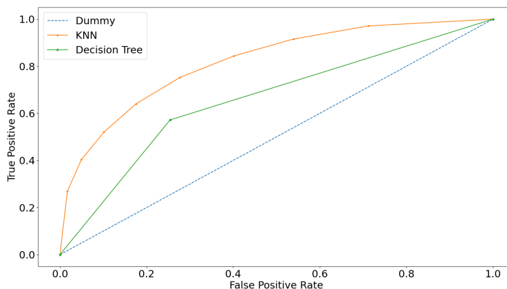
FIGURE 7: ROC curve for TWINE (Round 1-8) experiment ( AUROC_{KNN} = 0.818 , AUROC_{DT} = 0.659 )
