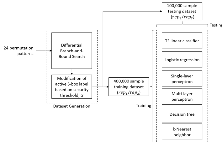
FIGURE 2: Experiment 1 - Phase 1/Phase 2 flow
