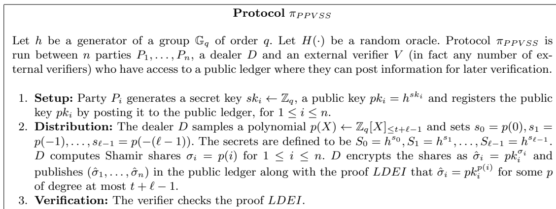
Fig. 5. Protocol \pi_{PPVSS}
