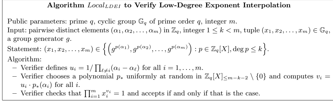
Fig. 3. Algorithm Local_{LDEI} to Verify Low-Degree Exponent Interpolation
