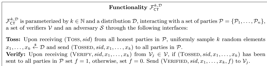
Fig. 10. Functionality \mathcal{F}_{CT}^{k,D} for G.O.D. Publicly Verifiable Coin Tossing.
