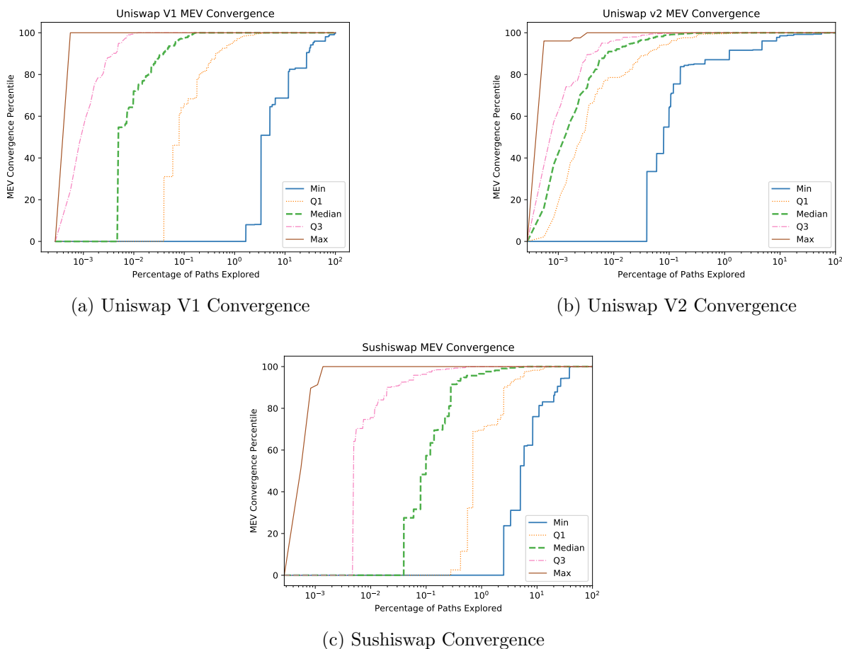
Figure 12: Convergence towards the optimal MEV for a random sample vs percentage of total paths explored for tractable blocks.
