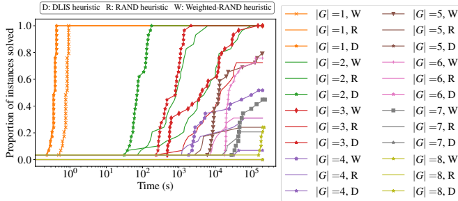
Figure 5: Haplotype benchmarks for when |G| \in [1..8] and r = 2|G| with timeout of 200k seconds. With all heuristics the solver is successful on small formulas, e.g. , |G| \leq 2 , for which DLIS outperforms the randomized heuristics. Weighted-RAND becomes the most effective for larger databases.
