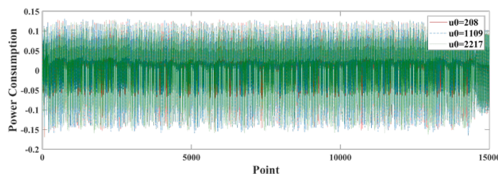
Fig. 8. Measurement traces of Listing 3 using three chosen ciphertexts (Optimization Level 3)
