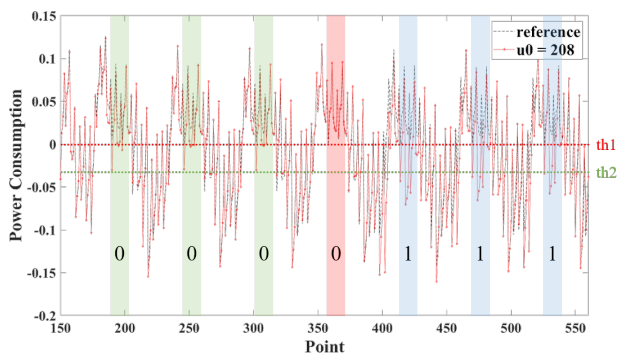
Fig. 4. A part of a power consumption trace of Listing 2 when we set ciphertext as \mathbf{u} = (208, 0) and v = 0 (Optimization Level 3)
