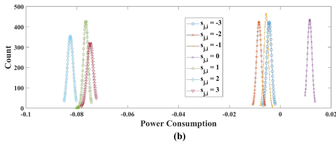
Fig. 10. Distributions of the PoIs when we set ciphertext as \mathbf{u} = (208, 0) and v = 0 ; (a) 383 point and (b) 387 point (Optimization Level s)
