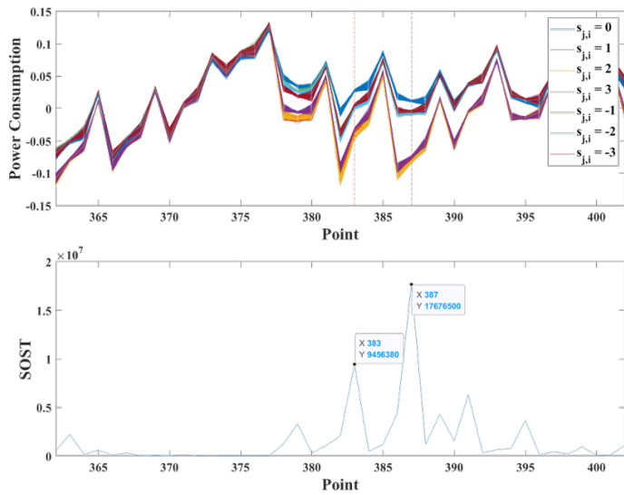
Fig. 9. The SOST values when we set ciphertext as \mathbf{u} = (208, 0) and v = 0 (Optimization Level s)
