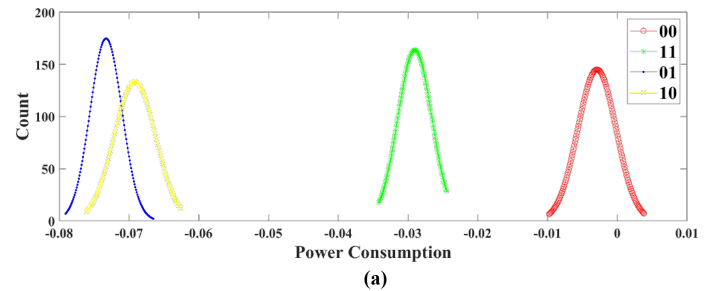
Fig. 12. Power consumption traces when we set ciphertext as \mathbf{u} = (208, 0) and v = 0 (m4 scheme, Optimization Level 3)
