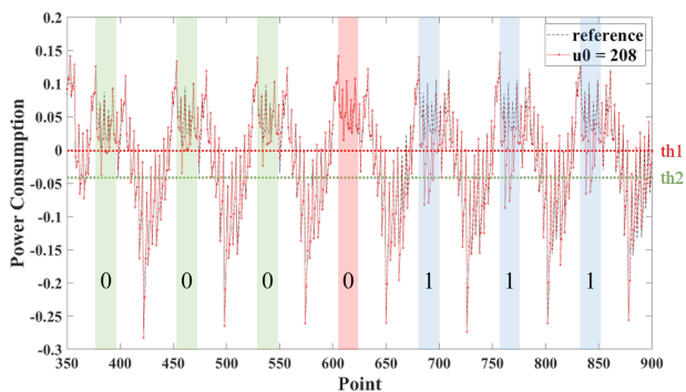
Fig. 5. A part of a power consumption trace of Listing 2 when we set ciphertext as \mathbf{u} = (208, 0) and v = 0 (Optimization Level 3)
