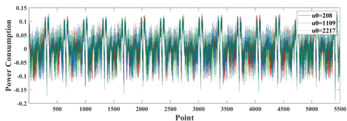
Fig. 14. Measurement traces of Listing 7 using three chosen ciphertexts (m4 scheme, Optimization Level 3)
