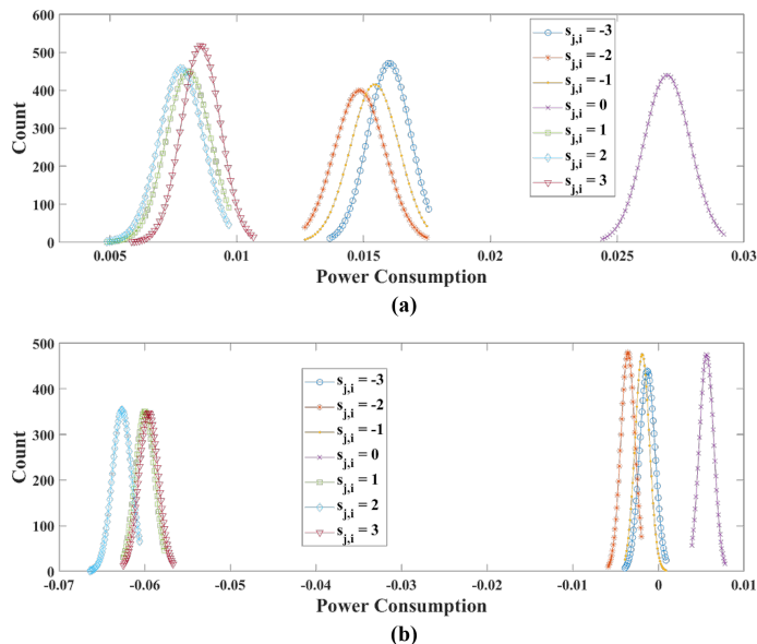
Fig. 7. Distributions of the PoIs when we set ciphertext as \mathbf{u} = (208, 0) and v = 0 ; (a) 191 point and (b) 195 point (Optimization Level 3)
