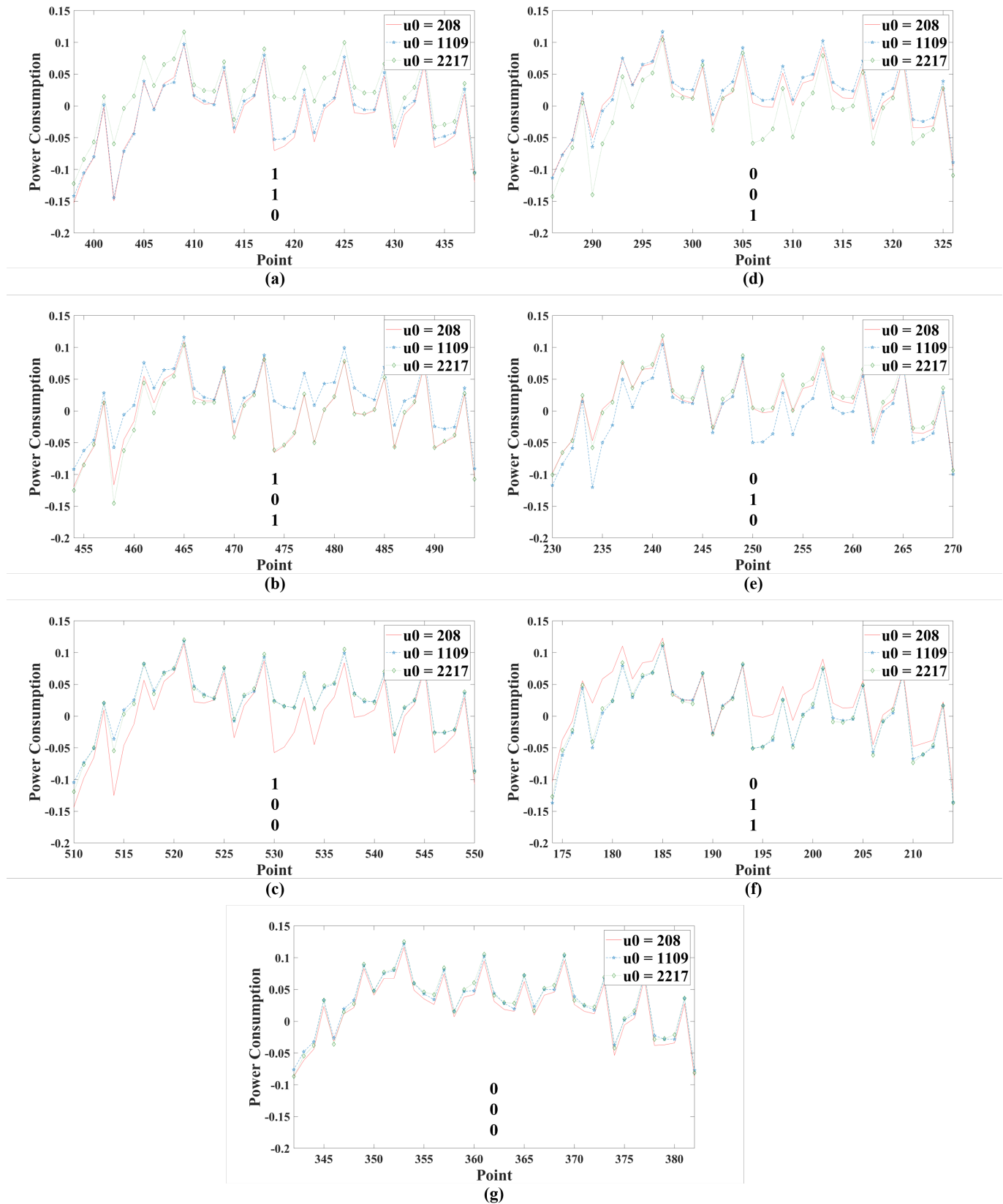
Fig. 15. Measurement traces using three chosen ciphertexts when (a) s_{0,i} = 1 , (b) s_{0,i} = 2 , (c) s_{0,i} = 3 , (d) s_{0,i} = -1 , (e) s_{0,i} = -2 , (f) s_{0,i} = -3 , and (g) s_{0,i} = 0 (Optimization Level 3).
