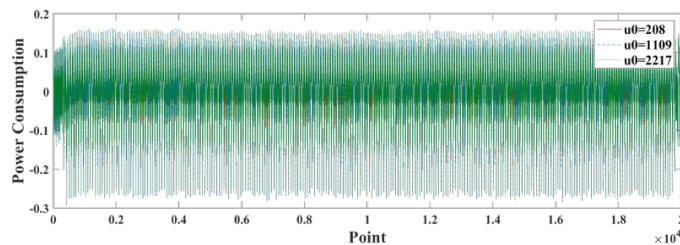
Fig. 11. Measurement traces of Listing 3 using three chosen ciphertexts (Optimization Level s)
