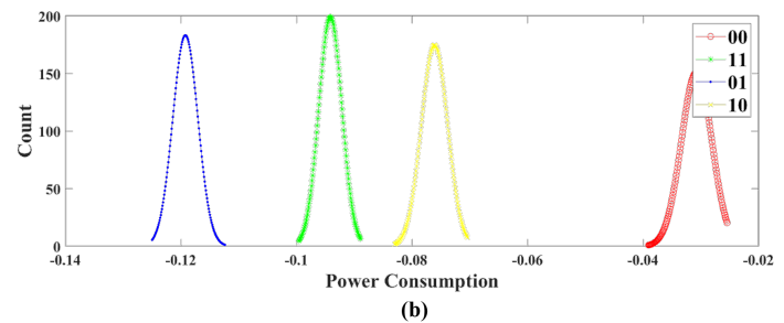
Fig. 13. Distributions of the PoIs when we set ciphertext as \mathbf{u} = (208, 0) and v = 0 ; (a) 31 point and (b) 35 point (m4 scheme, Optimization Level 3)
