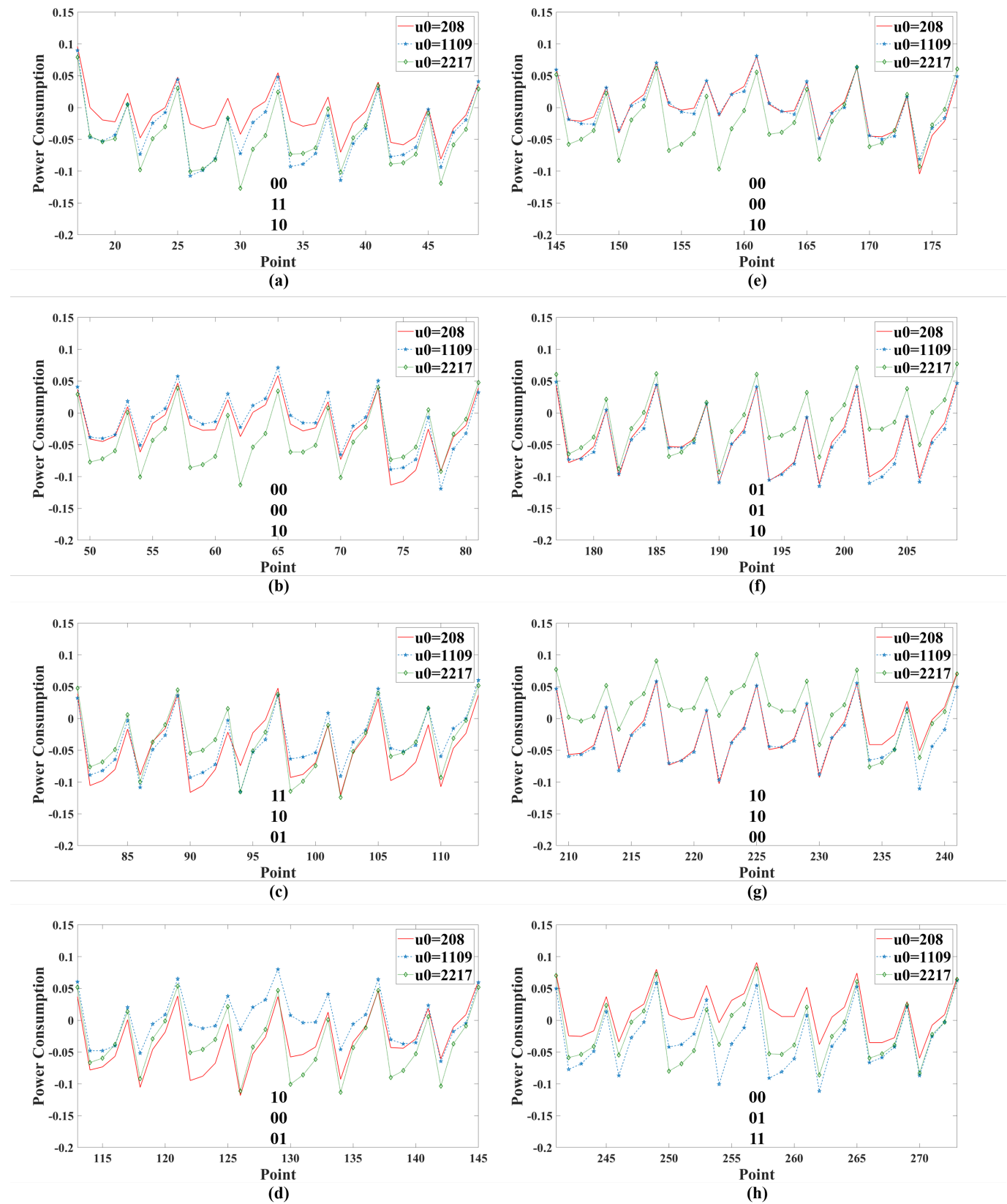
Fig. 17. Measurement traces using three chosen ciphertexts when (a) s_{0,i} = -3 , s_{0,i+1} = -2 , (b) s_{0,i} = -1 , s_{0,i+1} = 0 , (c) s_{0,i} = 1 , s_{0,i+1} = 2 , (d) s_{0,i} = 3 , s_{0,i+1} = -1 , (e) s_{0,i} = -1 , s_{0,i+1} = 0 , (f) s_{0,i} = -1 , s_{0,i+1} = 1 , (g) s_{0,i} = 1 , s_{0,i+1} = 0 , and (h) s_{0,i} = -1 , s_{0,i+1} = -3 (m4 scheme, Optimization Level 3)
