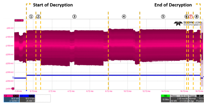
Fig. 3. Power consumption trace of Listing 1 (Optimization Level 3)
