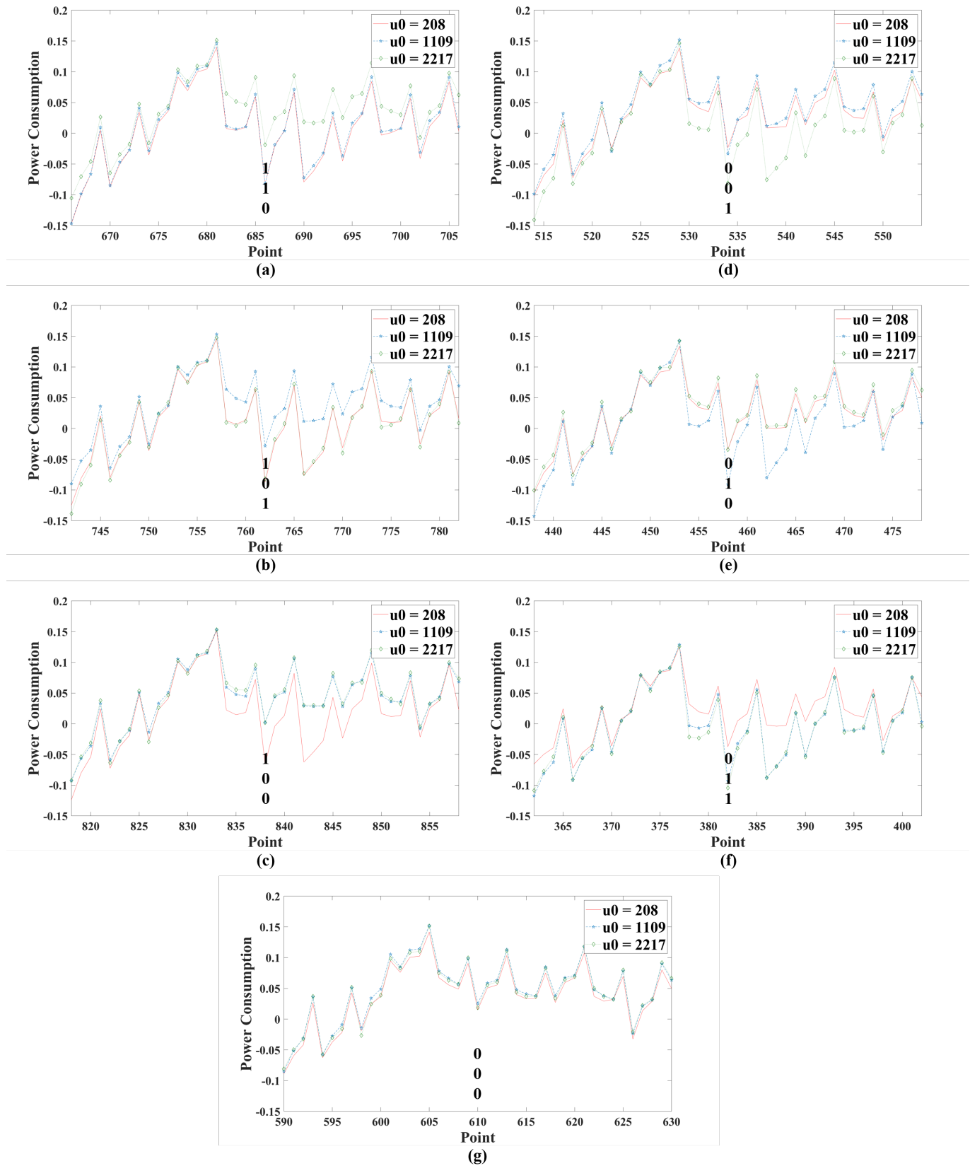
Fig. 16. Measurement traces using three chosen ciphertexts when (a) s_{0,i} = 1 , (b) s_{0,i} = 2 , (c) s_{0,i} = 3 , (d) s_{0,i} = -1 , (e) s_{0,i} = -2 , (f) s_{0,i} = -3 , and (g) s_{0,i} = 0 (Optimization Level s )
