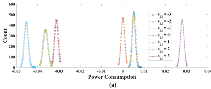
Fig. 12. Power consumption traces when we set ciphertext as \mathbf{u} = (208, 0) and v = 0 (m4 scheme, Optimization Level 3)
