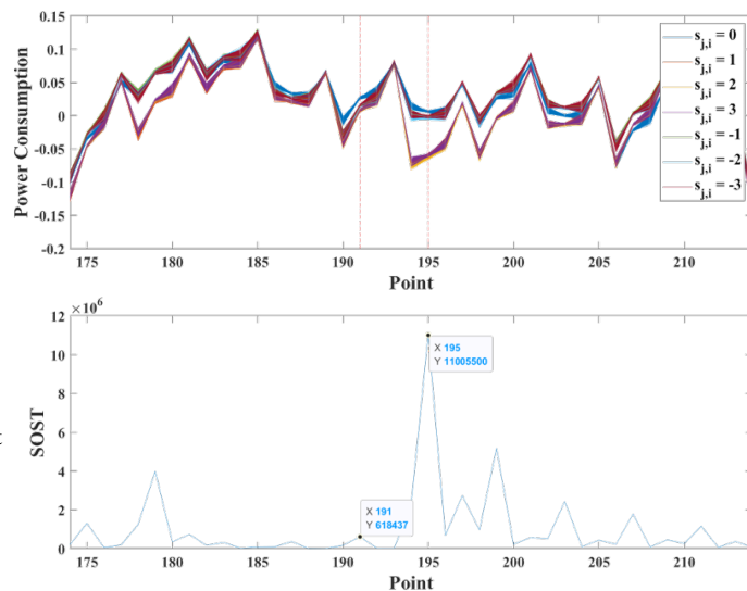
Fig. 6. The SOST values when we set ciphertext as \mathbf{u} = (208, 0) and v = 0 (Optimization Level 3)
