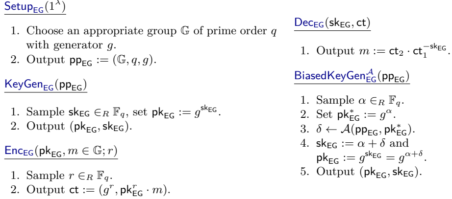
Fig. 21. Standard ElGamal encryption scheme and modified key generation \text{BiasedKeyGen}_{\text{EG}}^{\mathcal{A}} that allow an adversary \mathcal{A} to influence the distribution of public keys in a limited way.
