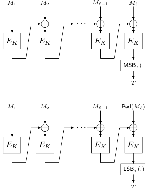
Fig. 3. The TrCBC construction. The first figure is for the full block messages, i.e., the message length is a multiple of the block size n , and the second figure is for messages whose length is not a multiple of n . \text{Pad}(M_{\ell}) = M_{\ell} \parallel 10^{n-|M_{\ell}|-1} and \tau < n/2 .
