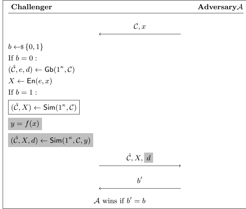
Fig. 3. Games for \text{ObvSim}_{\hat{\mathcal{G}}, \text{Sim}}^{\mathcal{A}} and \text{PrivSim}_{\hat{\mathcal{G}}, \text{Sim}}^{\mathcal{A}} . The steps in boxes only apply to \text{ObvSim} , and the highlighted steps only apply to \text{PrivSim} . Unmarked text means the steps appear in both games.
