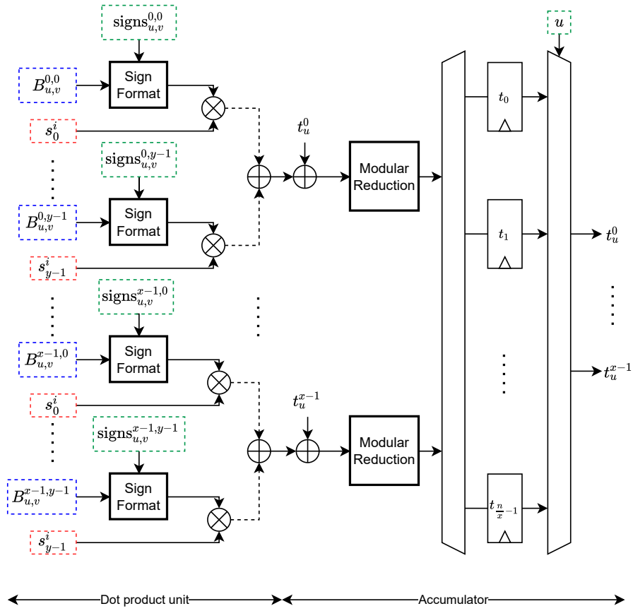
Fig. 4: Subproduct computation core and accumulator mechanism.
