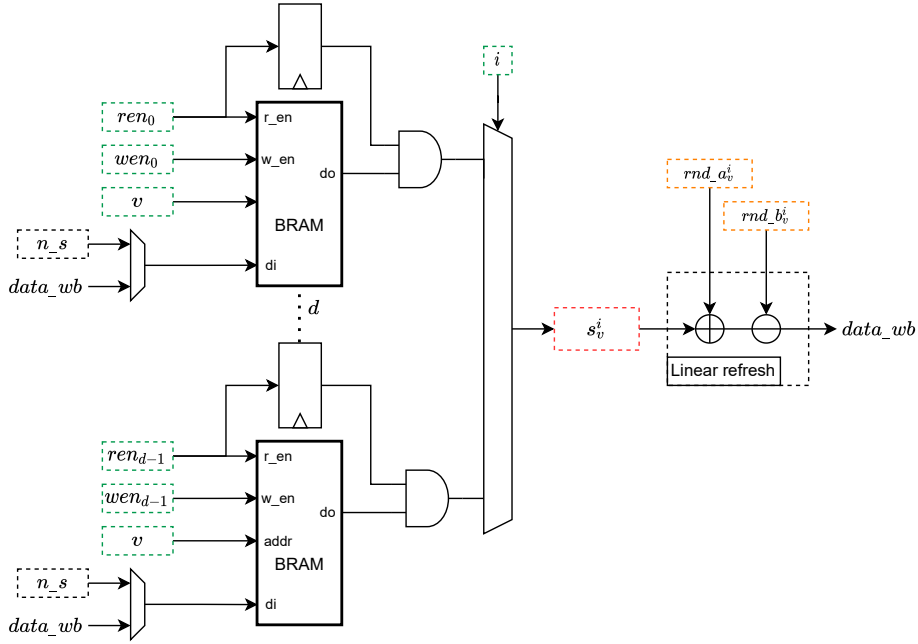
Fig. 5: Memory organization for the s_v^i storage.
