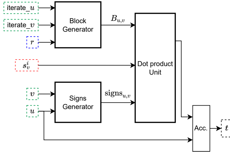
Fig. 3: Global architecture of our RLWPR prototype.
