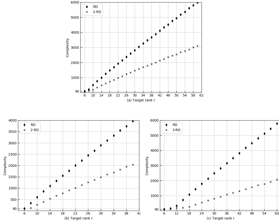
Fig. 1. Complexity trend of RD, 2-RD, and 3-RD by MM- \mathbb{F}_q .
