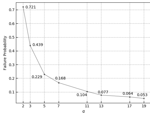
Fig. 7. Simulated failure probability of decoding the errors of weight \frac{n-k}{4} for 2-LRPC codes.
