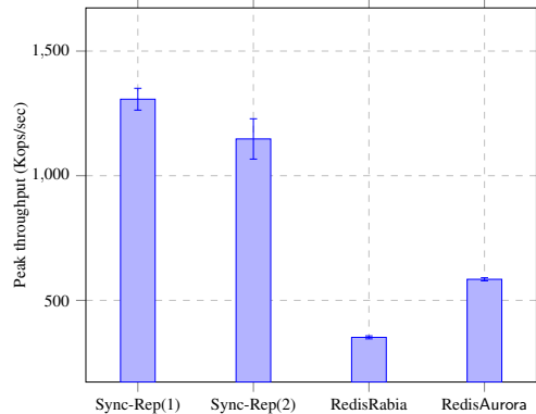
Figure 5: Throughput of different Redis integrations.
