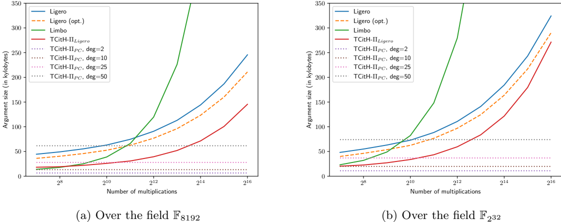
Fig. 4: Comparison of TCitH- \Pi_{PC} , TCitH- \Pi_{Ligerio} , Ligerio [AHIV17] and Limbo [DOT21] for arithmetic circuits (with input x \in \mathbb{F}^{100} ).
