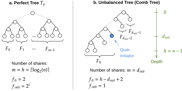
Figure 15: Default share distribution in a comb tree, that has the most depth-unbalanced possible structure, with a height h = n - 1 . In this case, the depth of the quarantine initiator is of primordial importance: the lower the initiator, the better the availability of a quarantine becomes.
