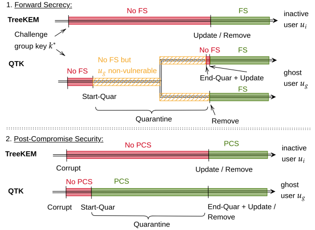
Figure 1: Comparison of the forward secrecy and post-compromise security of TreeKEM and our QTK protocol, with a focus on an inactive user that weakens the security of the entire group. Post-compromise security is achieved earlier with QTK and forward secrecy is enhanced by reducing the period of vulnerability of that inactive user.
