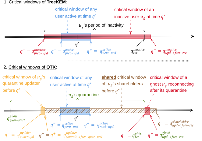
Figure 7: Compared critical windows, between TreeKEM and QTK, for the different types of users in a group, in the view of user u^* issuing a group key k^* at time q^* . The crosshatched brown box represents a shared critical window (cf. Definition 4.3), more secure than a proper one.
