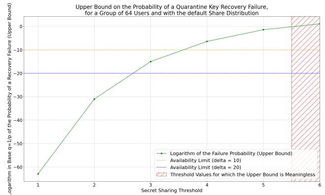
(b) Logarithmic Failure Probability with a Ratchet Tree of height h = 6
