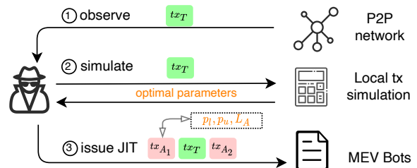
Fig. 1: Overview of JIT liquidity attack.
