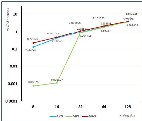
Figure 4: Total time spent in CPU seconds for verification (finding the related signatures from the blockchain, signature verification, decapsulation, and decryption).
