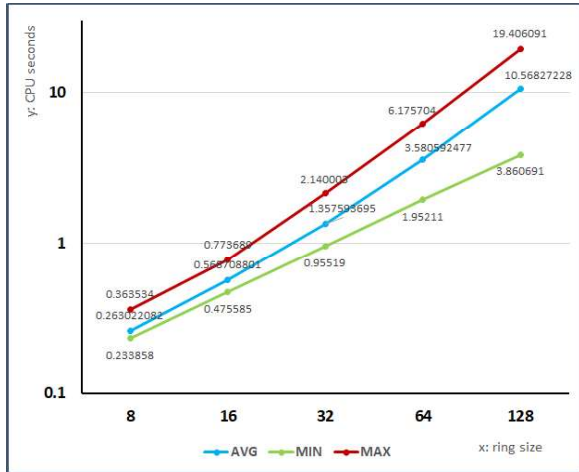
Figure 3: Total time spent in CPU seconds for block generation (signature file generation, traceability check, and block generation).
