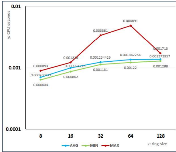
Figure 7: Time spent in CPU seconds for collecting related signatures for verification.
