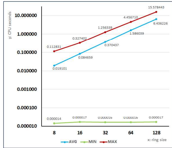
Figure 5: Time spent in CPU seconds for traceability check.
