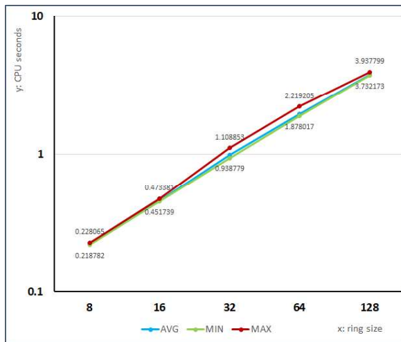
Figure 8: Time spent in CPU seconds for verification of a signature.
