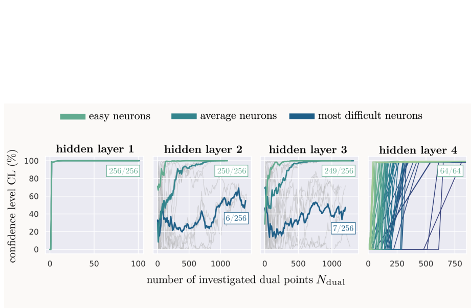
Fig. 11: The evolution of the sign recovery confidence level CL with the investigated number of dual points N_{dual} for easy neurons, average neurons, and the most difficult neurons in each layer.
