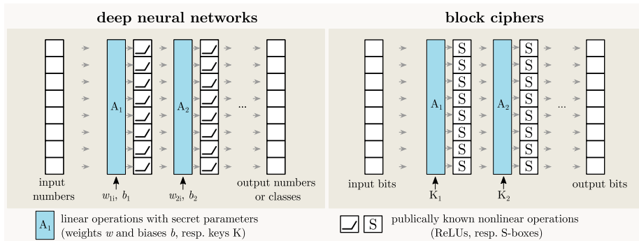
Fig. 1: The similarity between DNN’s and block ciphers.
