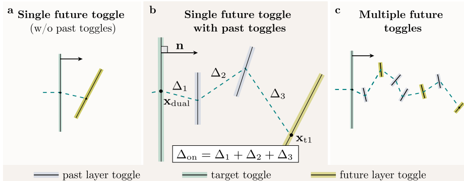
Fig. 7: Visualization of the distance measurement using the DISTANCETO_TOGGLE algorithm. a. In its simplest variant the distance measurement only accepts distance measurements from dual points at which the first toggle is a future layer toggle. b. A slightly more elaborate variant of the distance measurement handles past layer toggles by recomputing the decision hyperplane normal vector and continue moving until the first future layer toggle is encountered. c. In its most elaborate variant the distance measurement can gain statistics at a single dual point, by moving through multiple (instead of only a single) future toggle.
