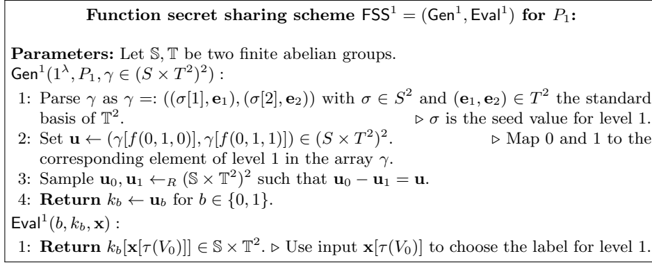
Fig. 5. FSS (\text{Gen}^1, \text{Eval}^1) for P_1 . Superscripts for k, s, t, v represent the party id.
