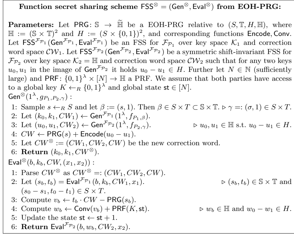
Fig. 1. FSS (\text{Gen}^\otimes, \text{Eval}^\otimes) for \mathcal{F}_{\mathcal{P}_1} \times \mathcal{F}_{\mathcal{P}_2} from \text{FSS}^{\mathcal{F}_{\mathcal{P}_1}}, \text{FSS}^{\mathcal{F}_{\mathcal{P}_2}} and EOH-PRG.
