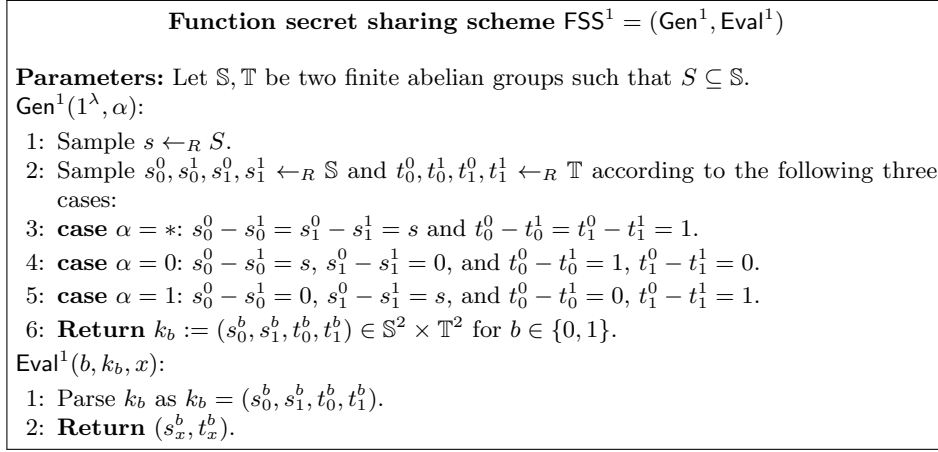
Fig. 4. One-bit FSS FSS^1 . Superscripts b for s and t represent the party id.
