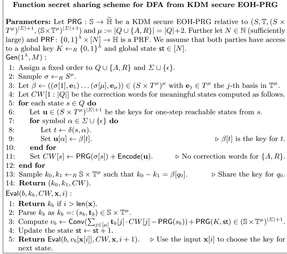
Fig. 3. FSS for a DFA from KDM secure EOH-PRG.
