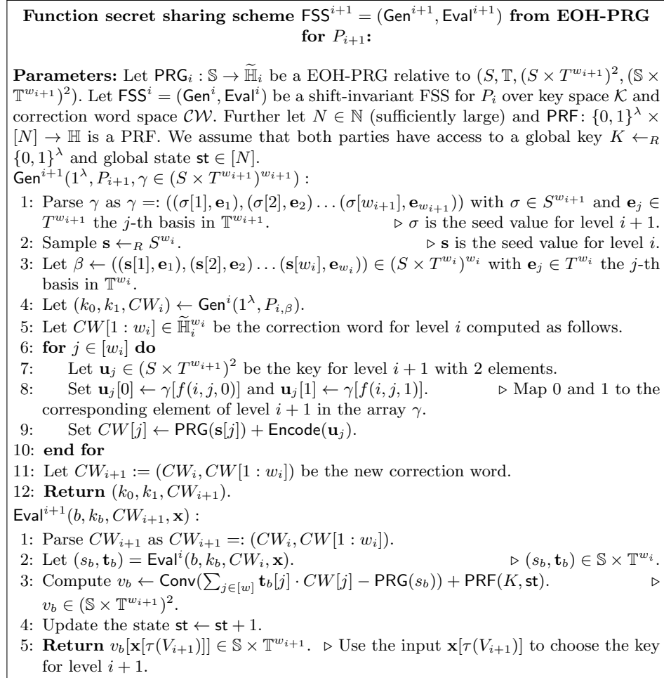
Fig. 2. FSS (\text{Gen}^{i+1}, \text{Eval}^{i+1}) for P_{i+1} from FSS (\text{Gen}^i, \text{Eval}^i) and EOH-PRG PRG.
