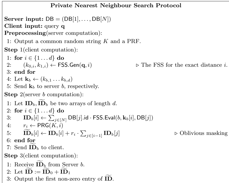
Fig. 6. Private nearest neighbour search protocol involving FSS for approximate matching function and oblivious masking.
