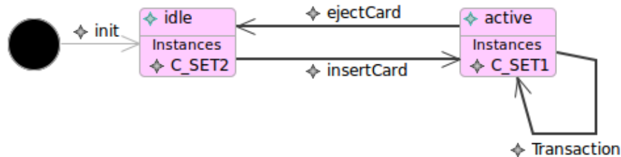
Fig. 1. State-machine Animation Example
