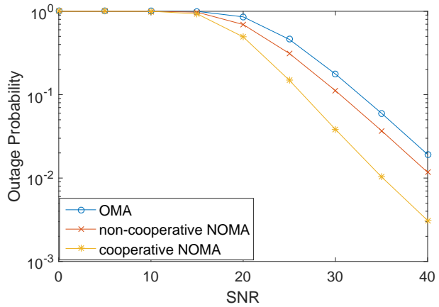
Figure 9: Performance comparison between cooperative NOMA and non-cooperative NOMA. The BS is located at (0, 0), User m is located at (4, 0), User n is located at (1, 0), the path loss exponent is 3, the power allocation coefficient for User m and User n are (0.8, 0.2). The targeted data rate is 1 bits per channel use (BPCU).
