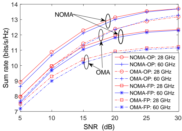
Figure 13: Illustration of the superiority of NOMA-mmWave over OMA-mmWave networks both at 28 GHz and 60GHz, “OP” refers to optimized power allocation, “FP” refers to fixed power allocation. The detailed parameter settings are found in [192].
