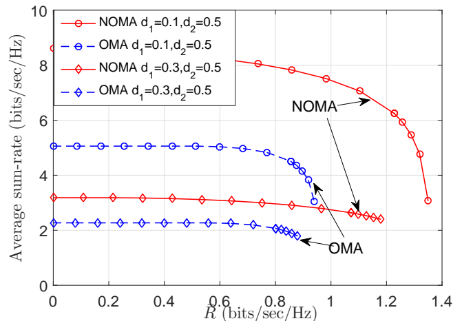
Figure 4: Illustration of the sum-rate versus the minimum rate constraints with full CSIT knowledge for different user distances. The full parameter settings can be found in [88].
