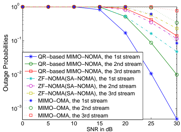
Figure 7: Comparison of MIMO systems with various multiple access techniques using a two-user case. M = N = 3 , where M is the number of antennas at transmitters, N is the number of antennas at receivers. As such, each user is to receive three data streams from the BS. R_m = 1.2 bit per channel use (BPCU) and R_n = 5 BPCU are the targeted data rates of User m and User n , respectively.
