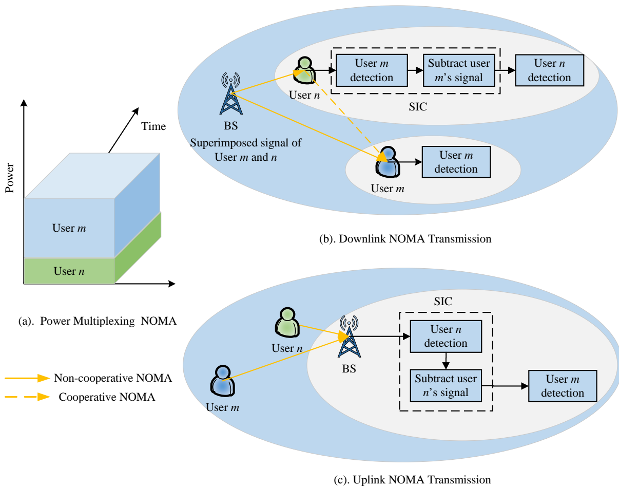
Figure 5: Illustration of NOMA transmission.
