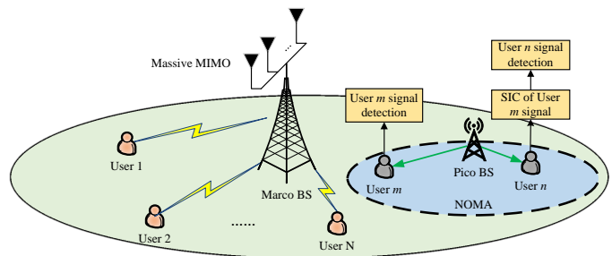
Figure 12: Illustration of NOMA and massive MIMO based hybrid HetNets.
