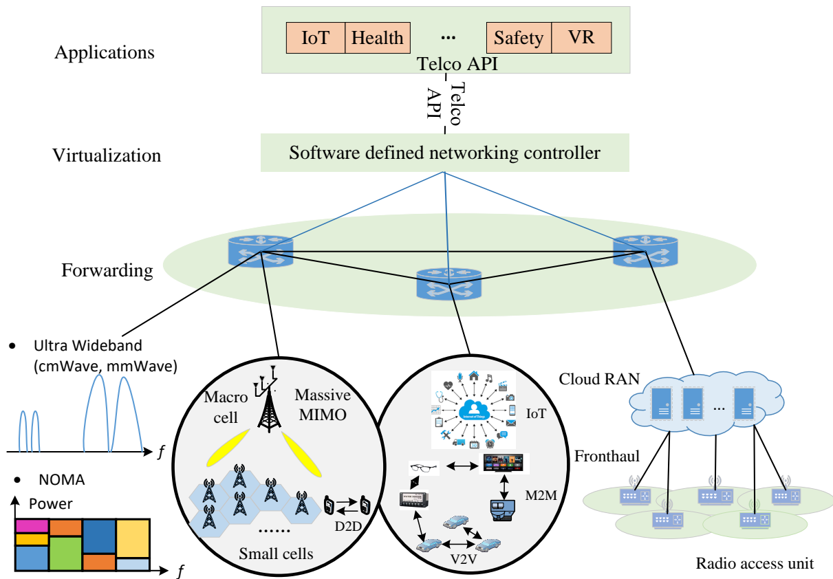
Figure 2: Illustration of the future 5G network architecture.
