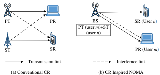
Figure 10: Comparison of convectional CR and CR inspired NOMA.
