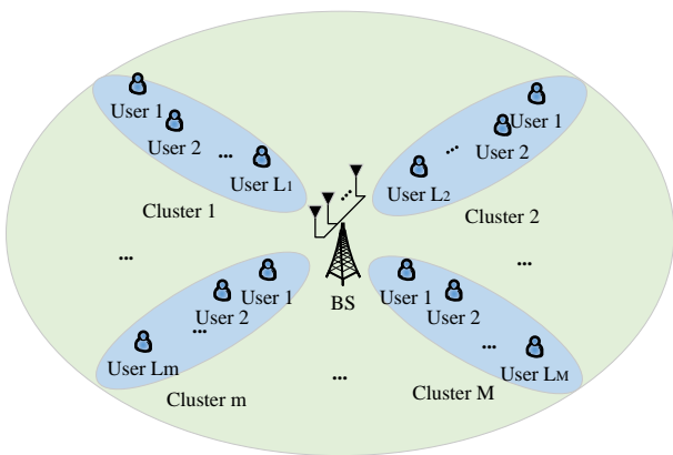
Figure 6: Illustration of cluster-based MIMO-NOMA.
