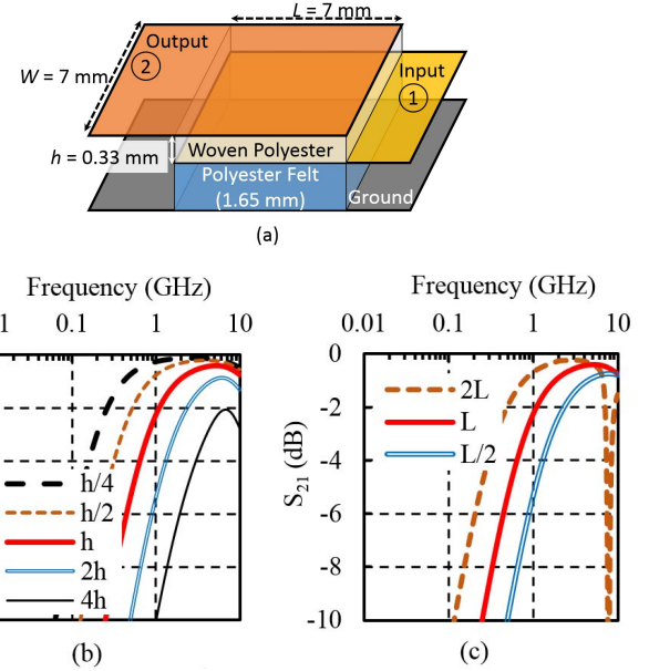
Fig. 9. Simulation of the broadside coupling performance. (a) 3-D view of the broadside-coupled microstrip lines. (b) S_{21} with variable h ( L = 7 mm). (c) S_{21} with variable L ( h = 0.33 mm).
