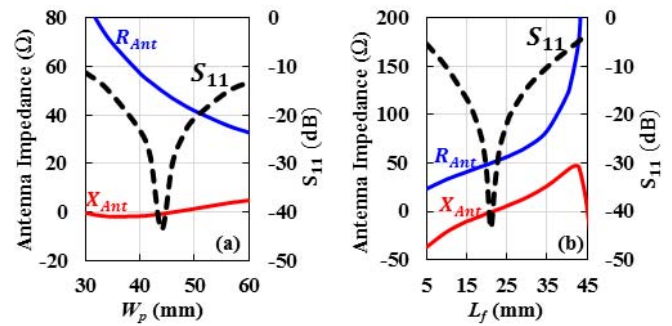
Fig. 6. Simulated antenna impedance, Z_{Ant} = R_{Ant} + jX_{Ant} , and input response S_{11} as function of the patch width W_p , and the length of the microstrip feed line L_f . (a) Variation of W_p with constant L_f = 21 mm. (b) Variation of L_f with constant W_p = 44 mm. The impedance of the antenna is calculated 10 mm from the edge of the patch in the x -axis direction, as shown in Fig. 7.
