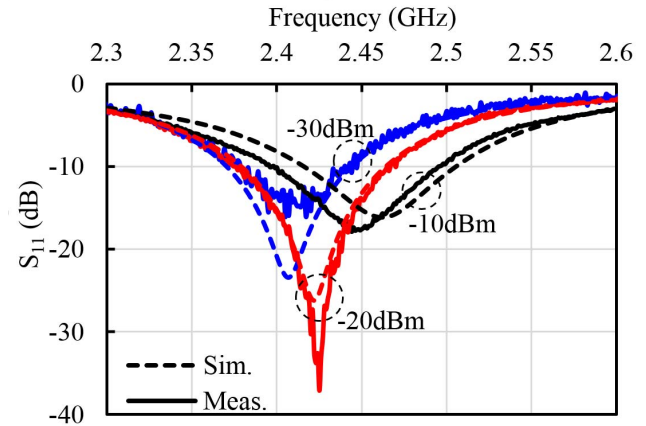
Fig. 18. Measured and simulated rectifier's input response at various power levels.
