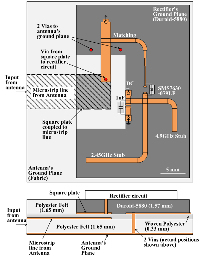
Fig. 11. Layout of the rectifier on Duroid-5880 ( 35 \times 23 mm) including the fabric-to-PCB coupling interface (top view is to scale). All vias are constructed from 0.3-mm radius metallic wire.
