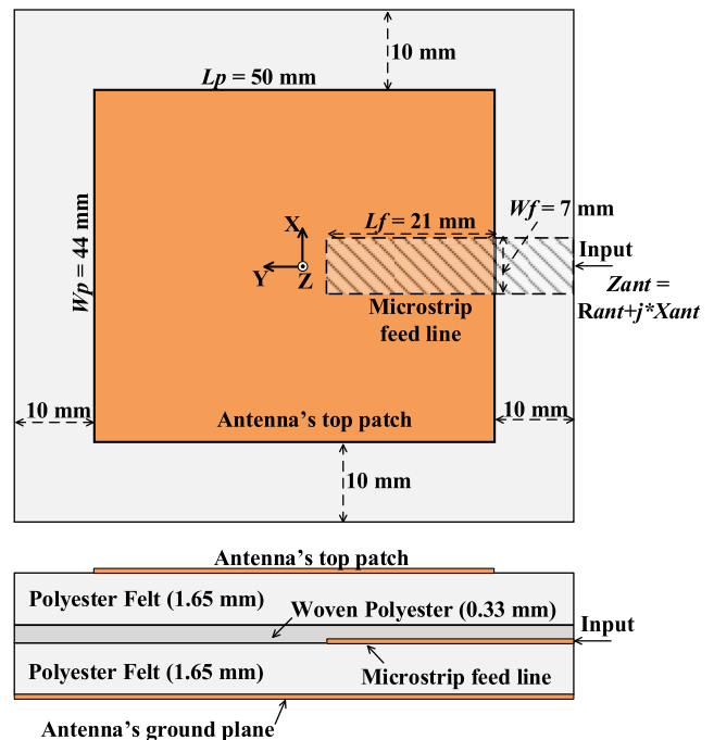
Fig. 7. Layout of the all-fabric antenna. All conductive parts are made from flexible copper fabric.
