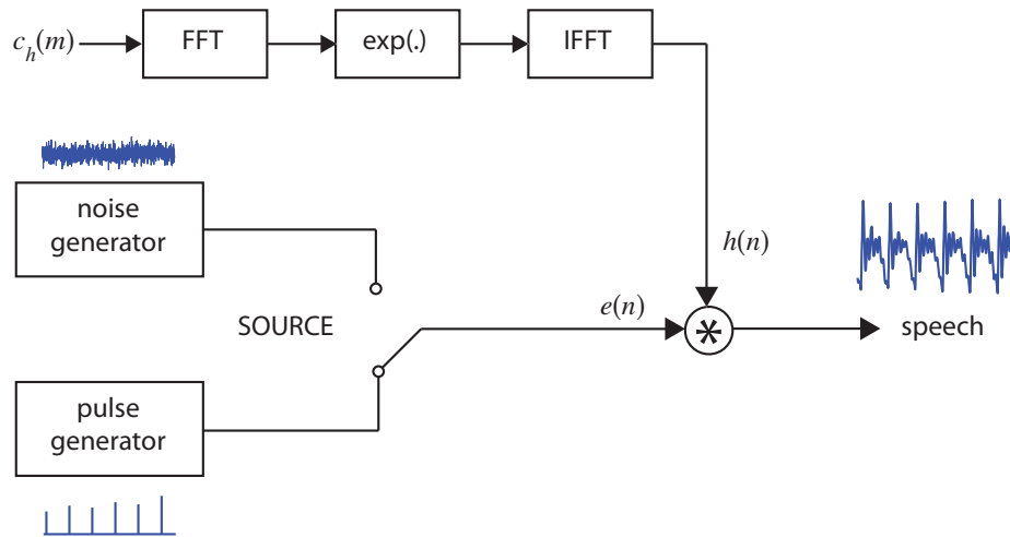
Figure 3.7: Cepstrum analysis.
