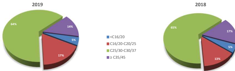
ERMCO Members - Production by strength class
