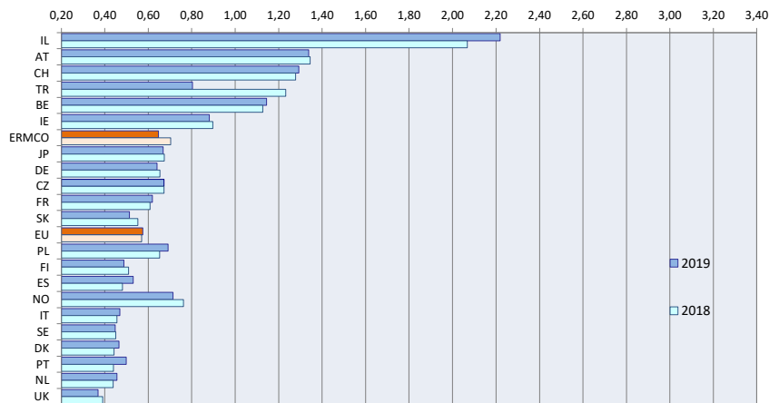
RMC unit production by country [m 3 /capita]
