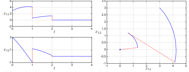
(a) The projections of trajectories of x_{11} and x_{12} on x_{11} and x_{12} respectively, the origin is denoted by the t direction. (b) Phase plot of x_{11} and x_{12} , the origin is denoted by the blue triangle.
