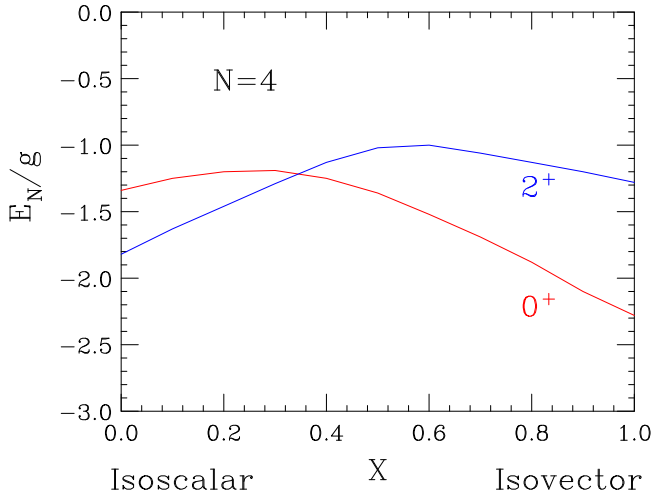
FIG. 1. Energies (in units of the pairing strength g ) of the lowest two T = 0 states for N = 4 particles in an f_{7/2} shell as a function of the relative mixture x of isovector and isoscalar pairing.
