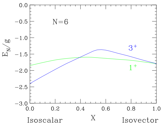
FIG. 2. Energies (in units of the pairing strength g ) of the lowest two T = 0 states for N = 6 particles in the f_{7/2} shell as a function of the relative mixture x of isovector and isoscalar pairing.
