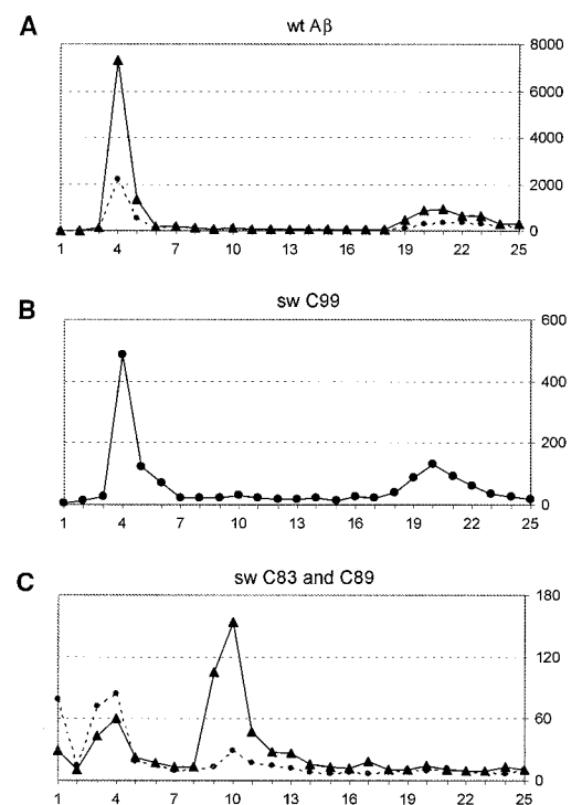
Fig. 6. Radiosequencing of BACE-induced APP metabolites. The figures show radioactivity in counts per min (cpm) per sequencing cycle. (A) Sequencing of A \beta from APPwt expressing cells transfected with BACE (triangles) or vector alone (circles and broken line) shows major peaks of 3 H-Phe in cycle 4, consistent with A \beta starting at Asp1. This cleavage is increased by BACE transfection. When the scale is expanded, secondary signals at cycles 7 and 10 indicative of Val-3 and Ile-6 cleavage are observed in the vector-alone transfectants (152 cpm and 97 cpm, respectively), but these signals are not increased upon BACE transfection (150 cpm and 110 cpm, respectively). (B) Sequencing of the 12 kD band from APPsw expressing cells that is induced upon BACE transfection (Fig. 5G) is consistent with an Asp1 start, indicating that this fragment is indeed C99, the immediate precursor of Asp1-A \beta . (C) Sequencing of the C83 and C89 COOH-terminal fragments from APPsw-expressing cells transfected with BACE (triangles) or vector alone (circles and broken line). Vector-alone transfectants show major peaks at cycles 1, 3, and 4, as expected for the previously reported Leu17 and Phe20 start sites of the \alpha -secretase product. BACE transfectants also show these C83 peaks, but the massively enhanced 11-kD band leads to strong signals in cycles 9 and 10, indicating a Glu11 cleavage product.
