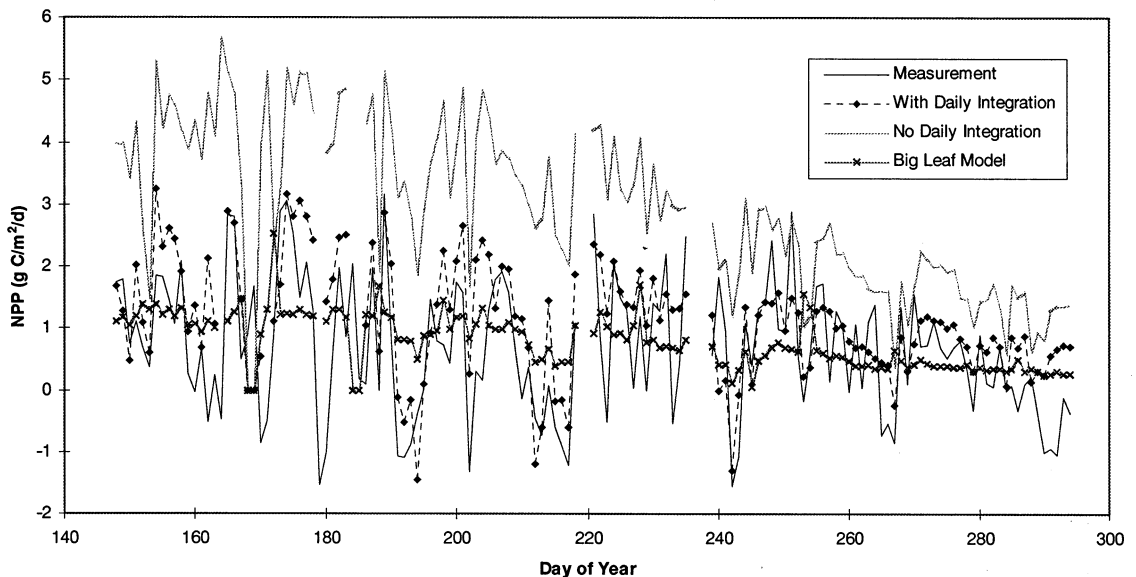
Fig. 6. Daily variations of overstory NPP obtained from tower and chamber measurements in comparison with modeled results. For all three modeling methodologies the same values were used for V_m , \Gamma and other coefficients in Farquhar's model. The same relationship between V_m and J_{\max} was also used.
