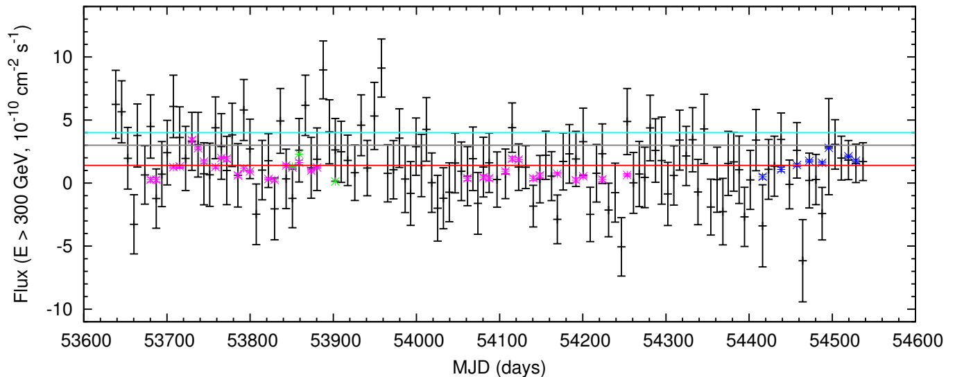
Fig. 3.— Light curve of Mrk 421 for energies above 300 GeV. In black: Milagro data; in magenta and in blue: data by Whipple and VERITAS respectively (Acciari et al. 2011); in green: MAGIC fluxes, calculated as the integral above 300 GeV of the measured spectra (Aleksić et al. 2010). Data from IACT observatories have been combined to match the Milagro time-binning. Also shown are in red the Milagro average flux ( 1.4 \times 10^{-10} \text{ cm}^{-2} \text{ s}^{-1} ), in grey and cyan the fluxes corresponding to the VERITAS mid and lowest high state (“high state A”) of Mrk 421 ( 3.1 \times 10^{-10} \text{ cm}^{-2} \text{ s}^{-1} and 4.1 \times 10^{-10} \text{ cm}^{-2} \text{ s}^{-1} respectively, calculated as the integral above 300 GeV of the corresponding best fit spectrum with a fixed cut-off energy of 4 TeV, see Acciari et al. 2011).
