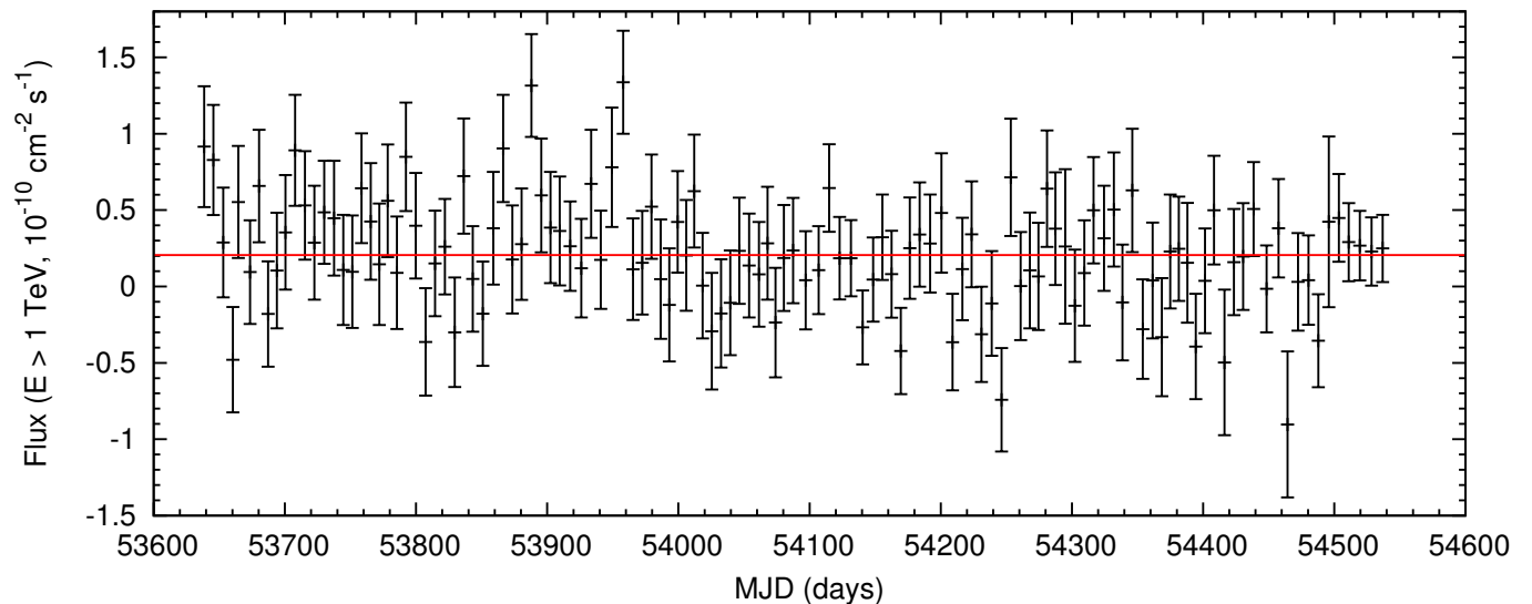
Fig. 2.— Light curve of Mrk 421 (black points) for energies above 1 TeV; the red solid line represents the average value of the flux: \bar{F}_{\text{Milagro}} = (0.205 \pm 0.030) \times 10^{-10} \text{ cm}^{-2} \text{ s}^{-1} . Each bin represents \sim 1 week of data.
