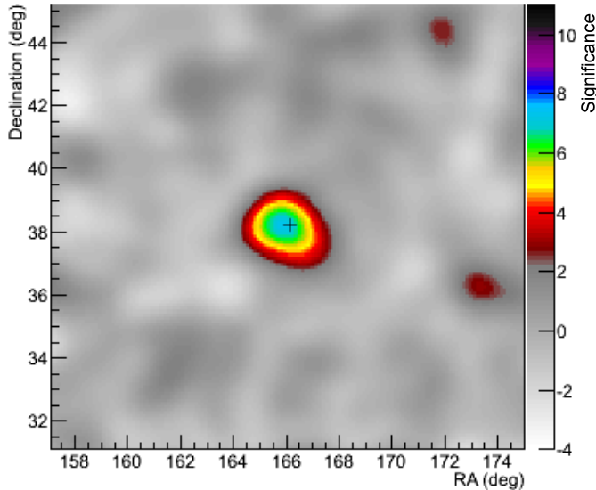
Fig. 1.— Sky map of the statistical significance in the region of Mrk 421. The significance at the Mrk 421 location (black cross) is 7.1 standard deviations.
