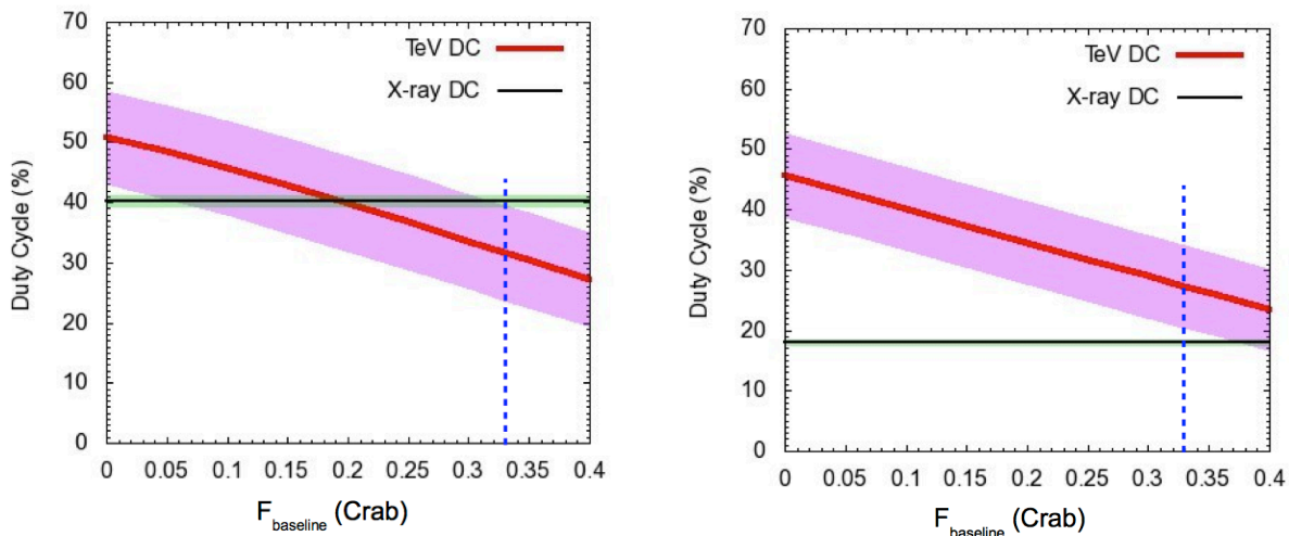
Fig. 6.— In red: TeV duty cycle calculated by considering as flares all the states having a flux above 1 TeV greater than F_{\text{baseline}}+N\sigma_G (left: N=1 , right: N=3 ); the shadowed pink area represents the error associated to the uncertainty on \bar{f} . In black: X-ray duty cycle, calculated by considering as flares all the states having a flux greater that R_{\text{char}}+N\sigma_{\text{char}} (left: N=1 , right: N=3 , Resconi et al. 2009); the shadowed green area represents its error. The dashed blue line marks the duty cycle values for F_{\text{baseline}}=0.33 Crab.
