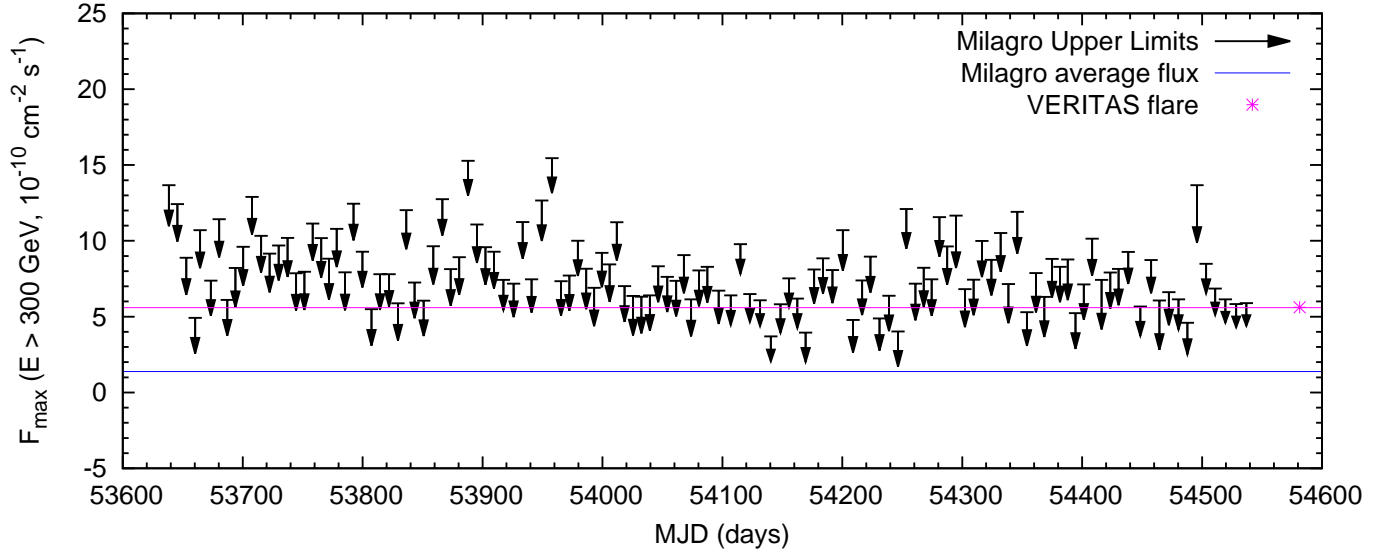
Fig. 4.— Black arrows: maximum averaged flux in a week time period for a flare in order to have not been detected at a 99.7 % C.L.; the length of the downward arrow for each point is the equal to the size of the corresponding error bar on the flux. Blue solid line: average Milagro flux above 300 GeV. Magenta star: observation by VERITAS corresponding to a flaring state, see Acciari et al. (2011); VERITAS data have been combined to have a weekly time-binning. The magenta line marks the flux level of the VERITAS flare along the whole Milagro observation period.
