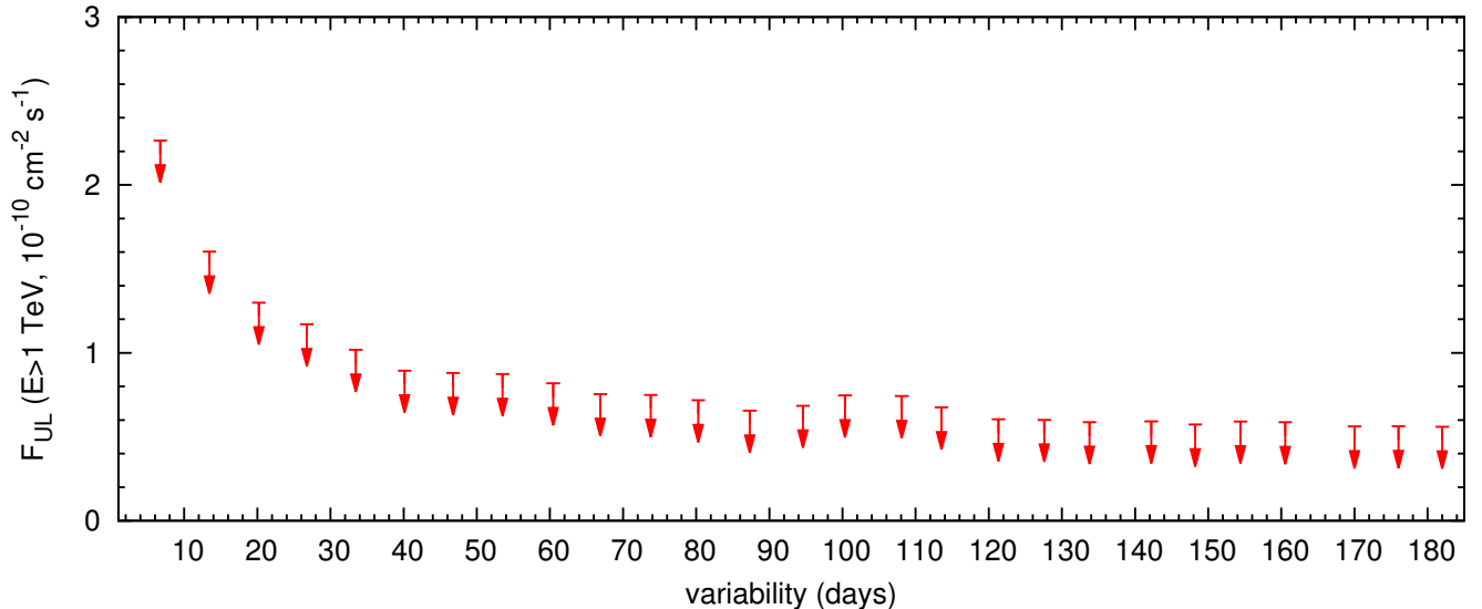
Fig. 5.— Upper limits on the flux as a function of the flare duration.
